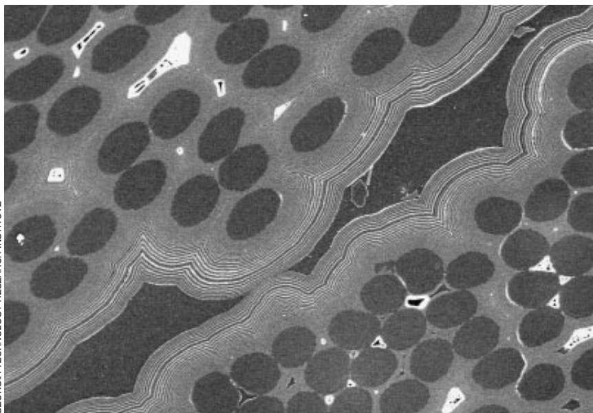
SILICON CARBIDE PLATELETS are laminated with ceramic layers through a process called chemical vapor infiltration.
